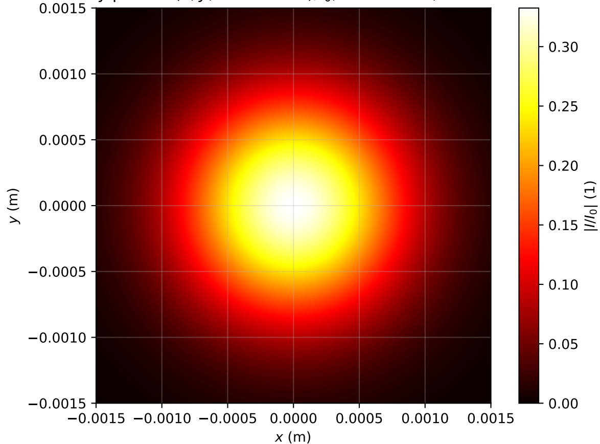
Intensity profile I(x, y, z = 3.025m)/I_0 , P_{in}=0.1P_{cr} , artificial time
